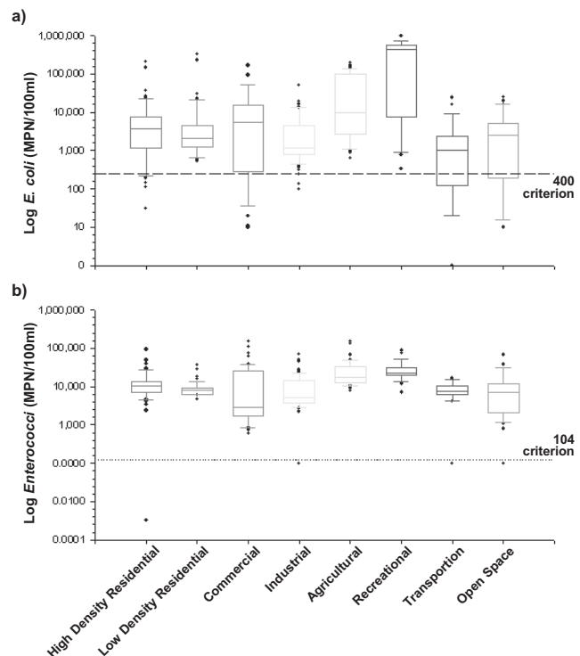
Figure 3. Distribution of Escherichia coli ( E. coli ; a) and enterococci (b) concentrations for the 2000 to 2005 wet seasons by land use type. Criterion lines = California State (single sample) water quality standards.
